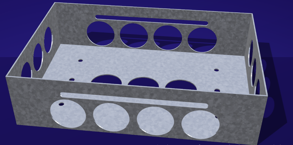
12M box, open face: punched entries and slots
